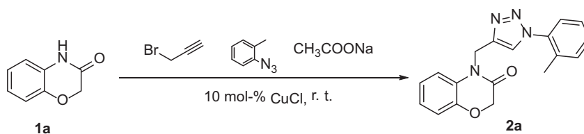
Scheme 1. The model reaction for the synthesis of 2a .
