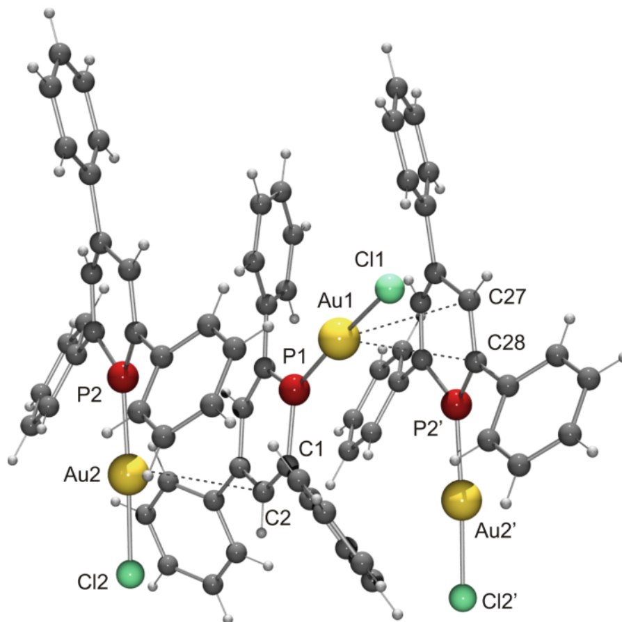
Fig. 2 (color online). Molecular structure and aggregation of [\text{AuCl}(\text{C}_5\text{H}_2\text{P-2,4,6-Ph}_3)] (two independent molecules) in the crystal. Intermolecular \text{Au}\cdots\pi interactions are indicated by dotted lines.
