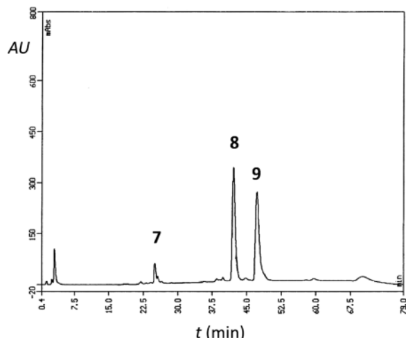
Fig. 1. HPLC elution profile of the crude reaction mixture after macrodimerisation of 7 [stationary phase: Macherey-Nagel EC 250/4 Nucleosil ® 100-5 SA (length 25 cm, diameter 1 cm, particle size 5 \mu\text{m} ); mobile phase: MeOH (10 min), then gradient MeOH to MeOH/NaOAc·3H 2 O (0.74 M) within 40 min, then MeOH/NaOAc·3H 2 O (0.74 M) for 10 min; flow rate 1 mL min -1 ; detection wavelength 250 nm].
