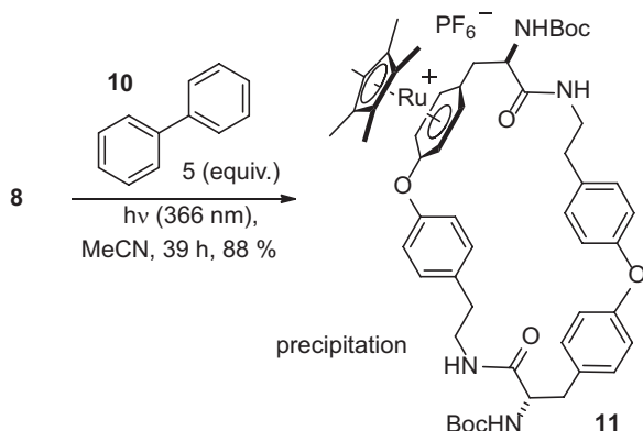
Scheme 3. Monodemetalation of the [RuCp*] + -complexed macrocycle 8 in the presence of biphenyl.
