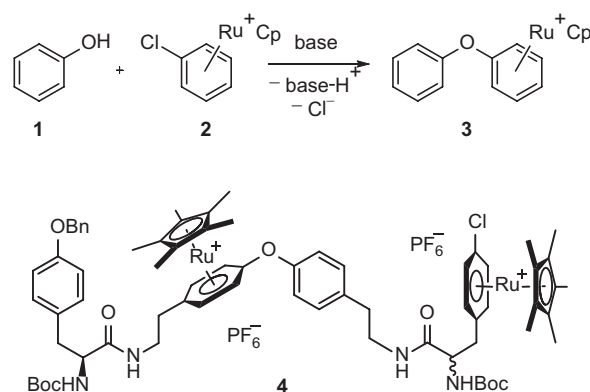
Scheme 1. Synthesis of Ru-complexed diaryl ether 3 by S N Ar reaction of phenolate and [CpRu] + -complexed chloroarene 2 ; dipeptide 4 equipped with two [RuCp*] + caps.
