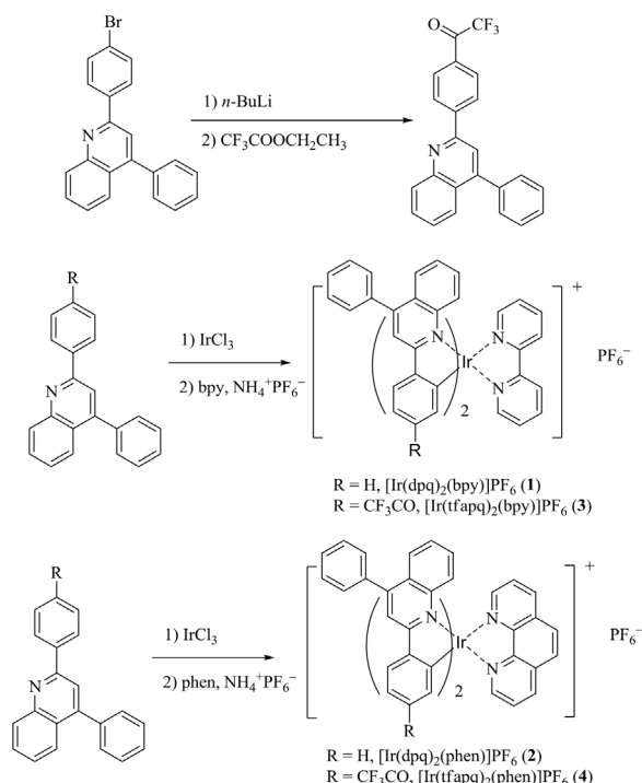
Scheme 1. Synthetic routes to iridium(III) complexes [\text{Ir}(\text{dpq})_2(\text{bpy})]\text{PF}_6 (1), [\text{Ir}(\text{dpq})_2(\text{phen})]\text{PF}_6 (2), [\text{Ir}(\text{tfapq})_2(\text{bpy})]\text{PF}_6 (3), and [\text{Ir}(\text{tfapq})_2(\text{phen})]\text{PF}_6 (4).
