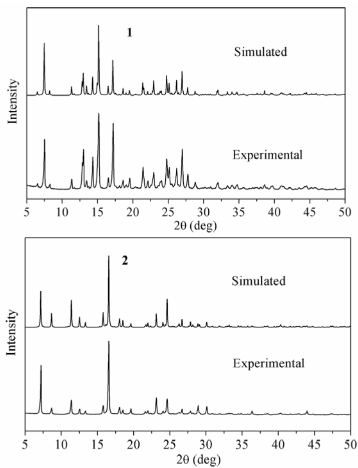
Fig. S1. Measured and simulated PXRD patterns for 1 and 2 .
