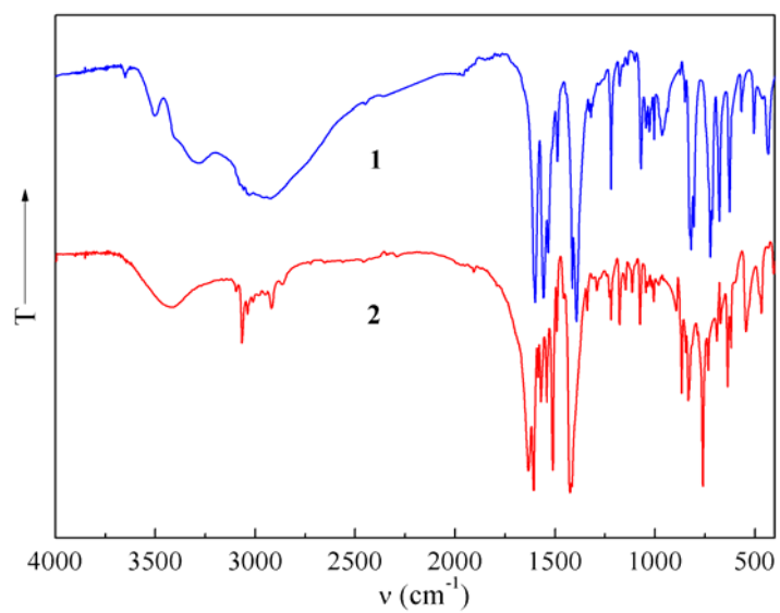
Fig. S2. Infrared spectra of 1 and 2 .
