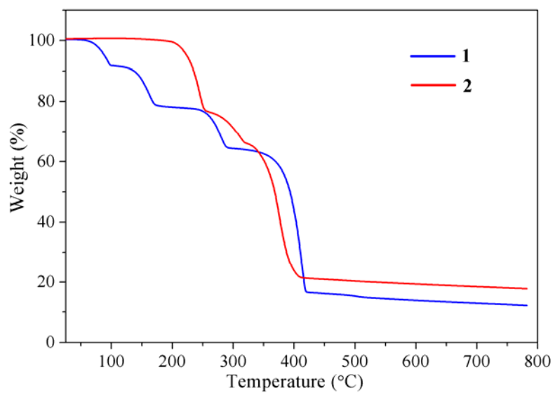
Fig. S3. Thermogravimetric curves for 1 and 2 .
