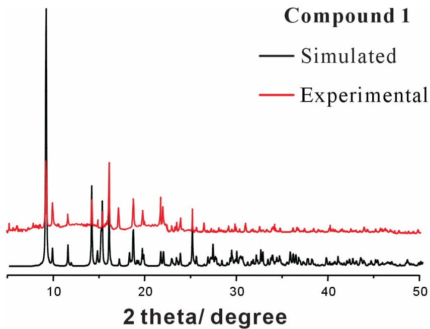
Figure S1. Observed and calculated PXRD patterns of 1 .
