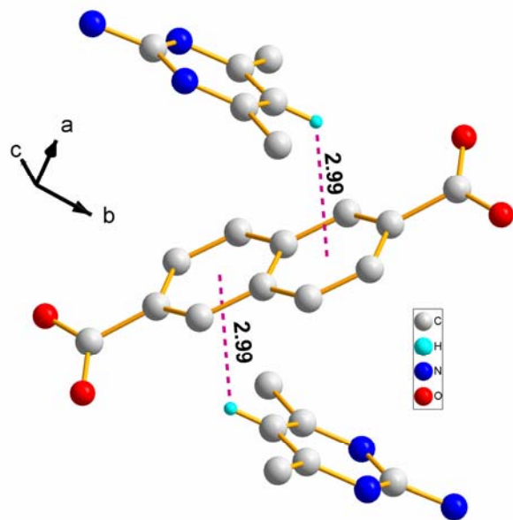
Figure S3. Representation of the C–H... \pi interactions in the crystal structure of 1 .
