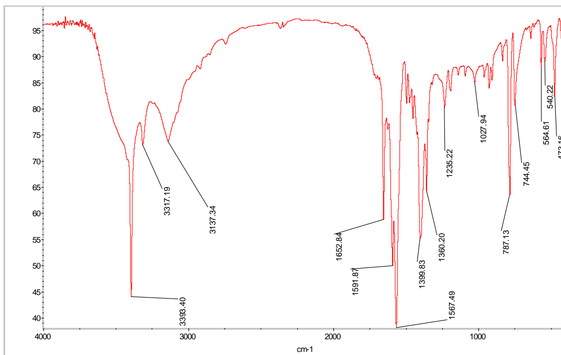
Figure S2. IR spectrum of 1 .
