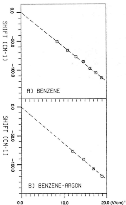
Fig. 1. a) Electric field dependence of the ionization threshold for benzene □ experimental values, --- least squares fit for a square root dependence. b) Electric field dependence of the ionization threshold for the benzene-Argon complex □ experimental values, --- least squares fit for a square root dependence.
