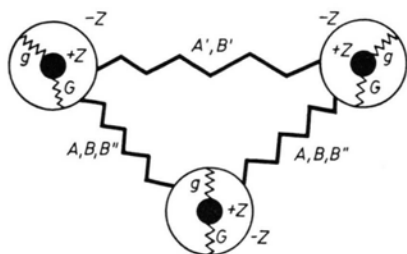
Fig. 1. Force constants of a breathing shell model for a face-centered cubic crystal. A, B nearest neighbour force constants, B' non-central part of B , A', B' second nearest neighbour force constants, Z core charge (= -shell charge), G shell-core dipole spring, g shell-core breathing spring.
